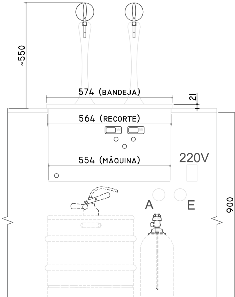
VISTA FRONTAL
